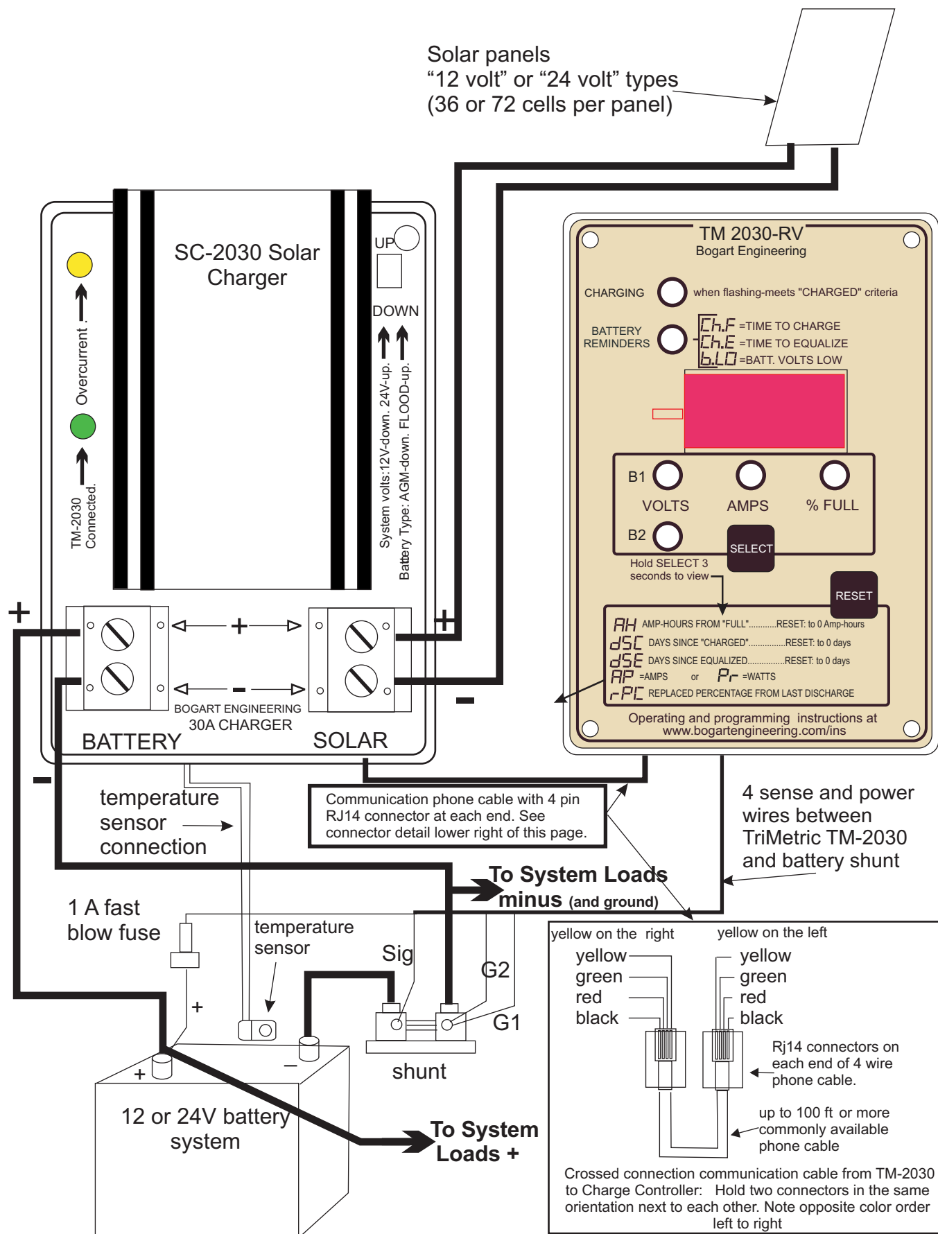
Wiring for TriMetric TM2030 and charge controller--not showing circuit breakers to battery or solar panels Figure 1
